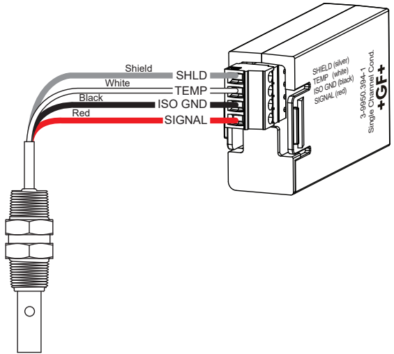
Single Channel Conductivity Module
