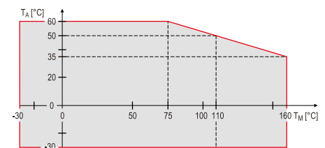
Ambient temperature (T A ) vs. process temperature (T M )
